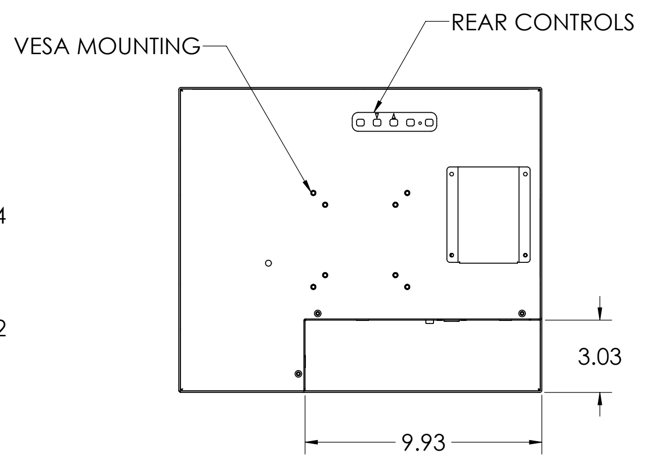
REAR VIEW
